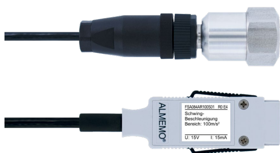
Vibration sensor FSA 084-xx with ALMEMO® connector
